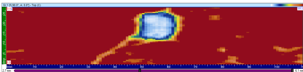
Figure 4. Ultrasonic C-scan images for \text{SiO}_2 /rubber/epoxy CFRC typical sample.
